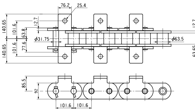
RF320-T-K1 Attachment Chain
