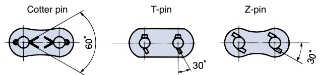
Fig. 11 Opening range of pins
