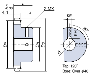
Hub without groove (14T and over)
