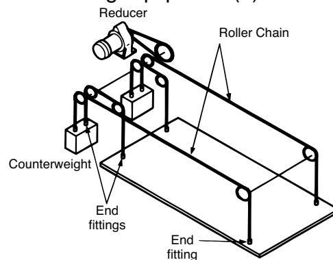
Lifting equipment (3)
