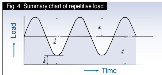
Fig. 4 Summary chart of repetitive load
