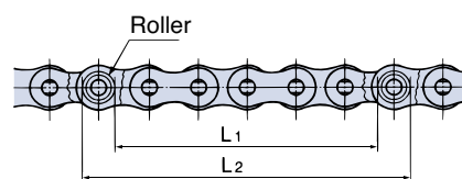
Fig. 28 Measuring length
