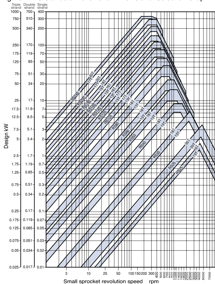
Figure 2: RS Standard Roller Chain Provisional Selection Graph
