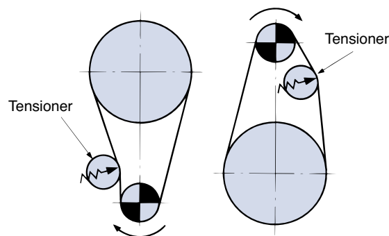
Fig. 22 Vertical transmission
