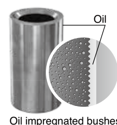
Oil impregnated bushes
