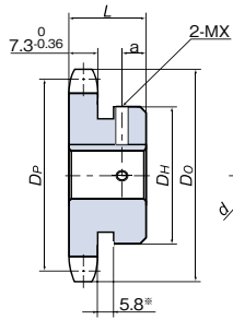
Hub with groove (10T – 12T)
