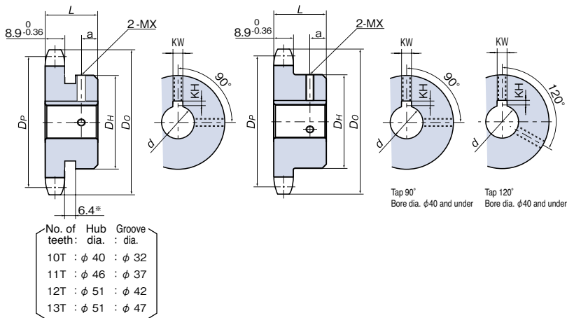
Hub with groove (10T – 13T)
