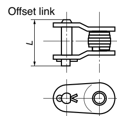
Connecting link RS80-SNS-1: Cotter pin-type
