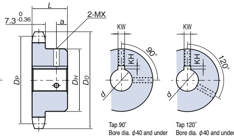
Hub without groove (13T and over)
